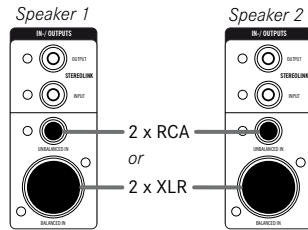
fig. 1: Common connection
