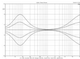
Abb. 10: Shelve Filter
